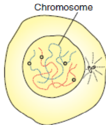
A Prophase
